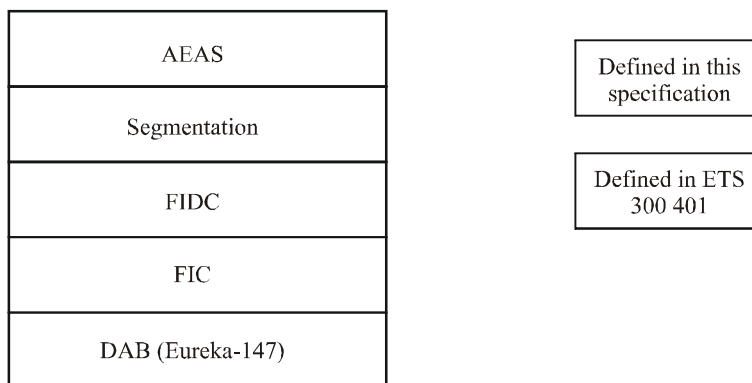
Protocol stack for the automatic emergency alert service
